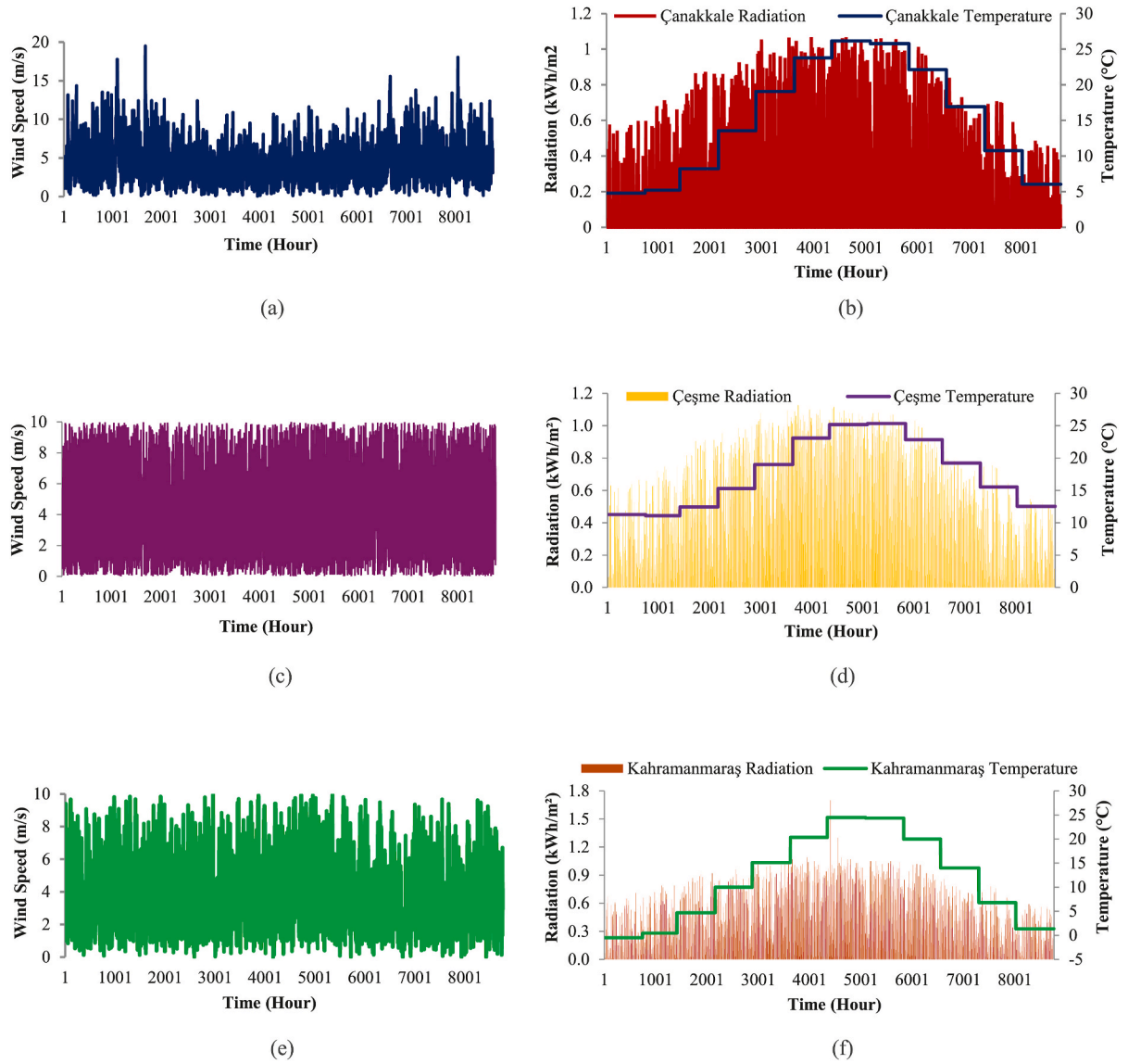
Fig. 2. Annual hourly data for three locations Wind speed data (a) Çanakkale (c) Çeşme (e) Kahramanmaraş Solar radiation and temperature data (b) Çanakkale (d) Çeşme (f) Kahramanmaraş.
