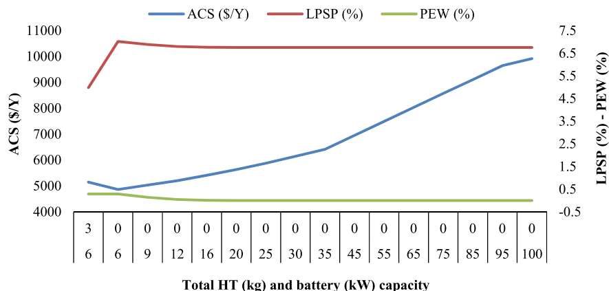
Fig. 25. The impact of HT absence and increased battery capacities on ACS, LPSP, and PEW. (Scenario 2 lowest ACS solution for Çeşme).
