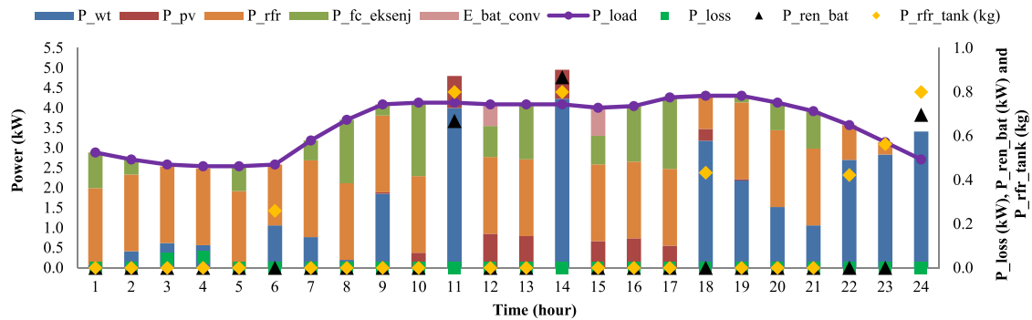
Fig. 16. Energy flow for Çeşme according to Scenario 2 of a winter day.
