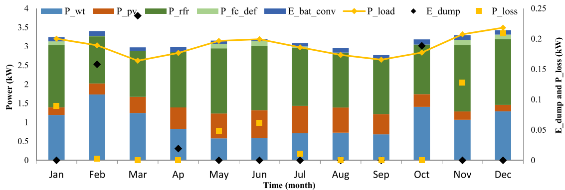
Fig. 11. Annually Energy flow, Wasted energy and loss of load for Çanakkale according to Scenario 2.
