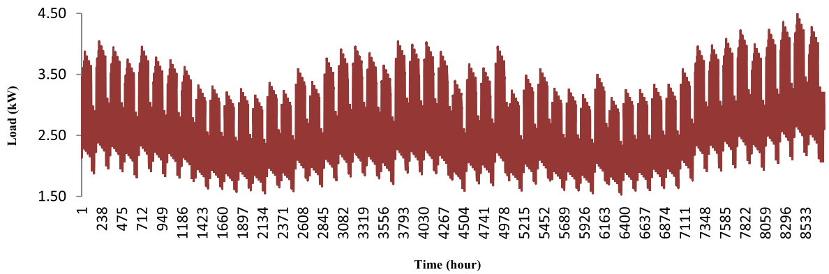
Fig. 3. Annual load data on hourly basis.
