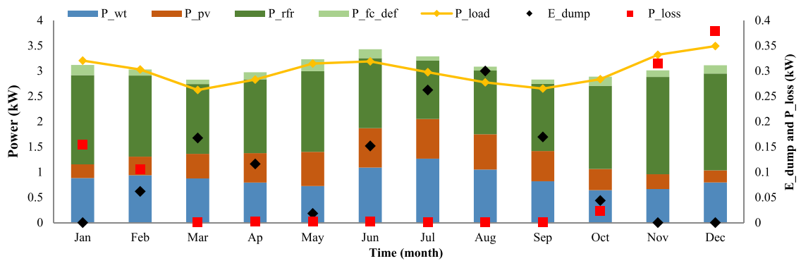
Fig. 17. Annually energy flow, wasted energy and loss of load for Kahramanmaraş according to Scenario 1.
