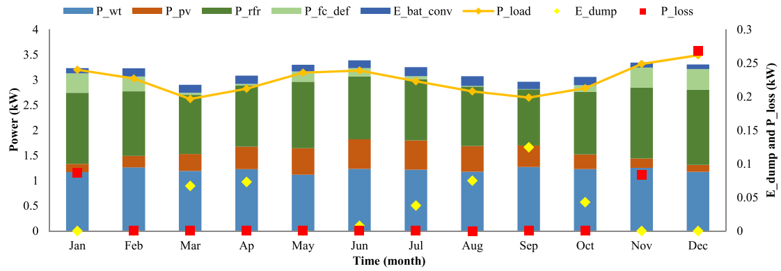
Fig. 15. Annually energy flow, wasted energy and loss of load for Çeşme according to Scenario 2.
