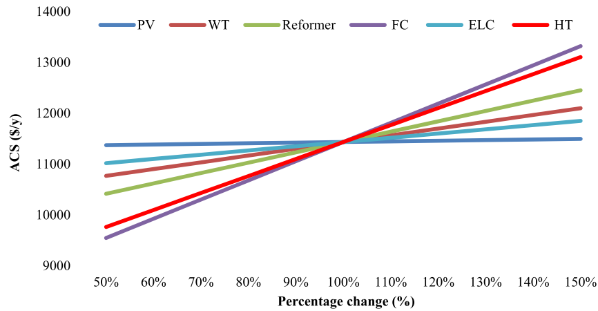
Fig. 21. Sensitivity of ACS to Cost Variations in PV, WT, fuel cell, electrolyzer, and HT (Scenario 1 lowest LPSP solution for Çanakkale).
