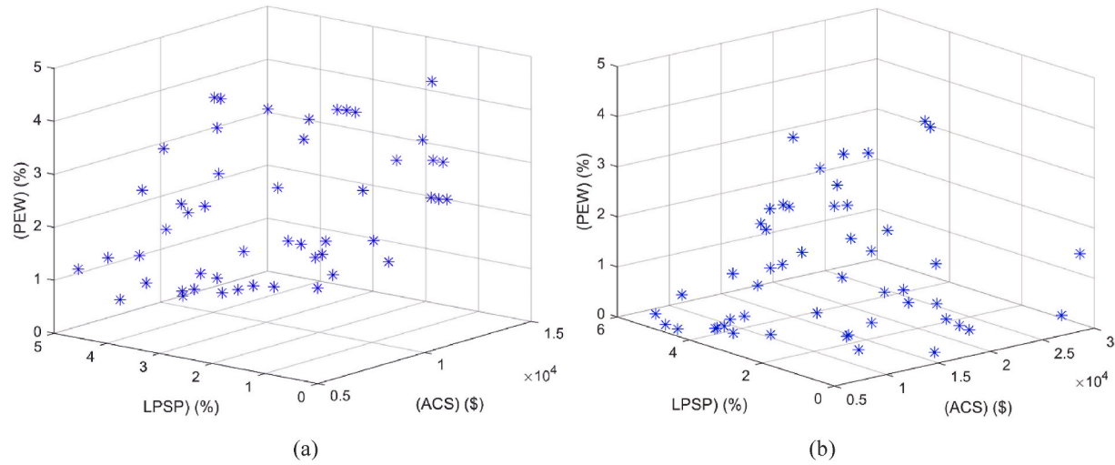
Fig. 7. The Pareto front for Çeşme (a) Scenario 1 (b) Scenario 2.
