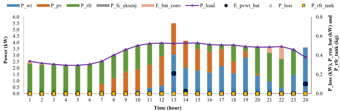
Fig. 20. Energy flow for Kahramanmaraş according to Scenario 2 of a summer day.
