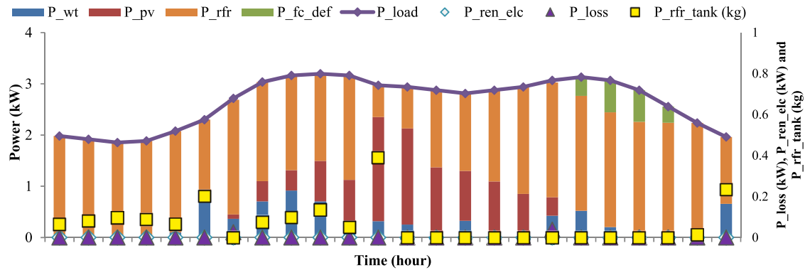
Fig. 10. Energy flow for Çanakkale according to Scenario 1 of an autumn day.
