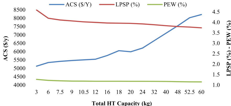
Fig. 23. The influence of increasing total HT capacity on ACS, LPSP, and PEW. (Scenario 1 lowest ACS solution for Çeşme).
