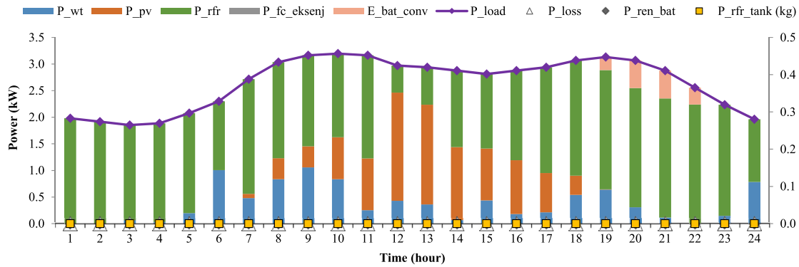
Fig. 12. Energy flow for Çanakkale according to Scenario 2 of an autumn day.
