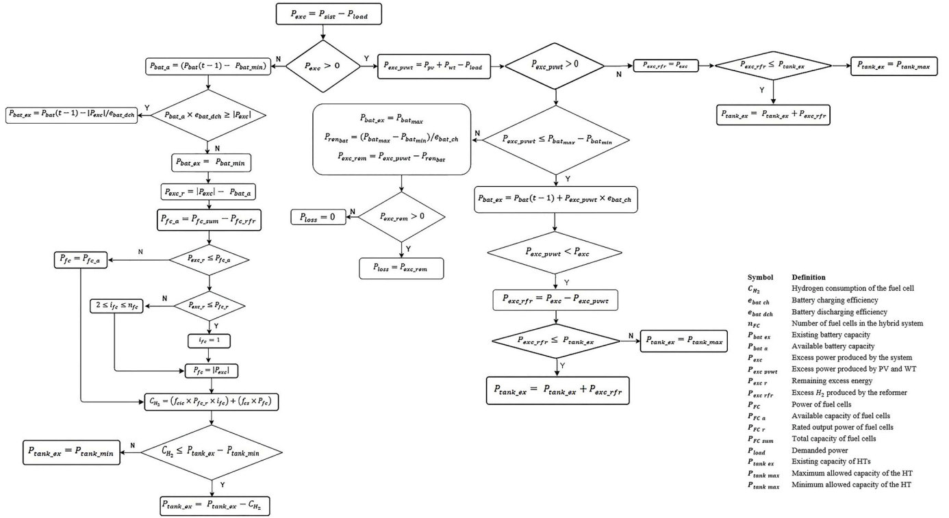
Fig. 5. A brief diagram of developed PMS.
