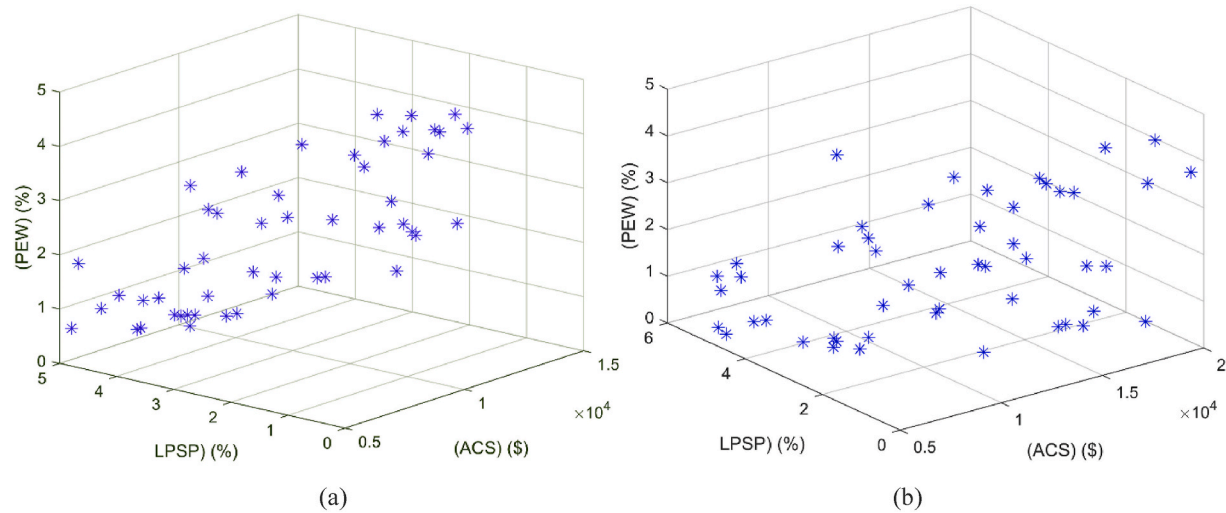
Fig. 6. The Pareto front for Çanakkale (a) Scenario 1 (b) Scenario 2.
