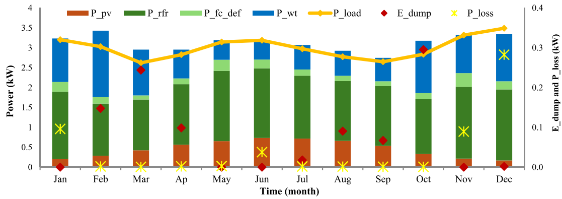
Fig. 9. Annually energy flow, wasted energy and loss of load for Çanakkale according to Scenario 1.
