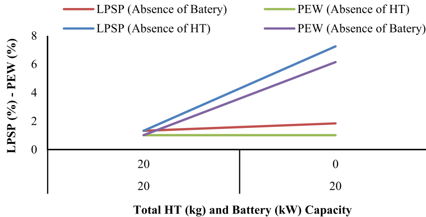
Fig. 26. The impact of the HT and the battery on LPSP and PEW.
