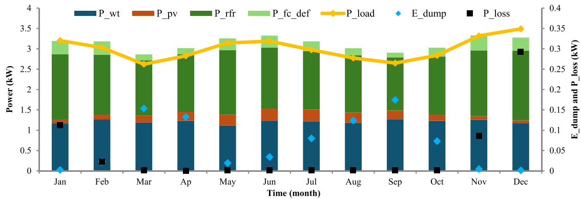
Fig. 13. Annually energy flow, wasted energy and loss of load for Çeşme according to Scenario 1.
