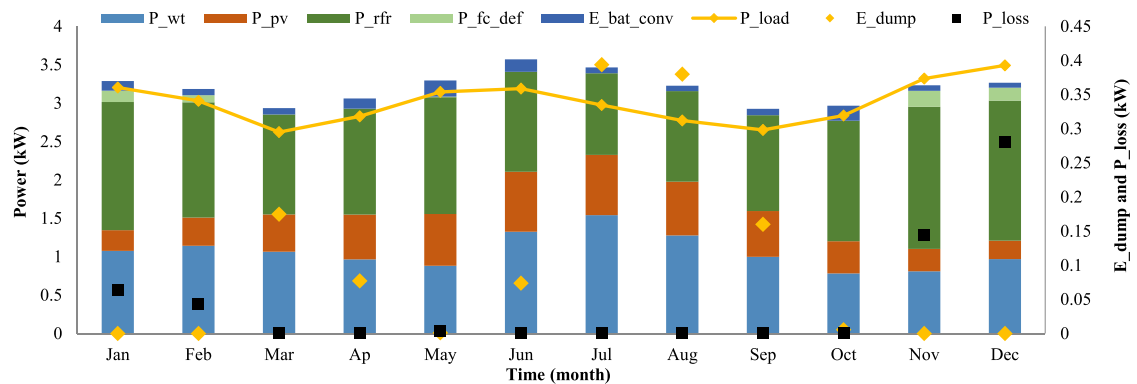
Fig. 19. Annually energy flow, wasted energy and loss of load for Kahramanmaraş according to Scenario 2.
