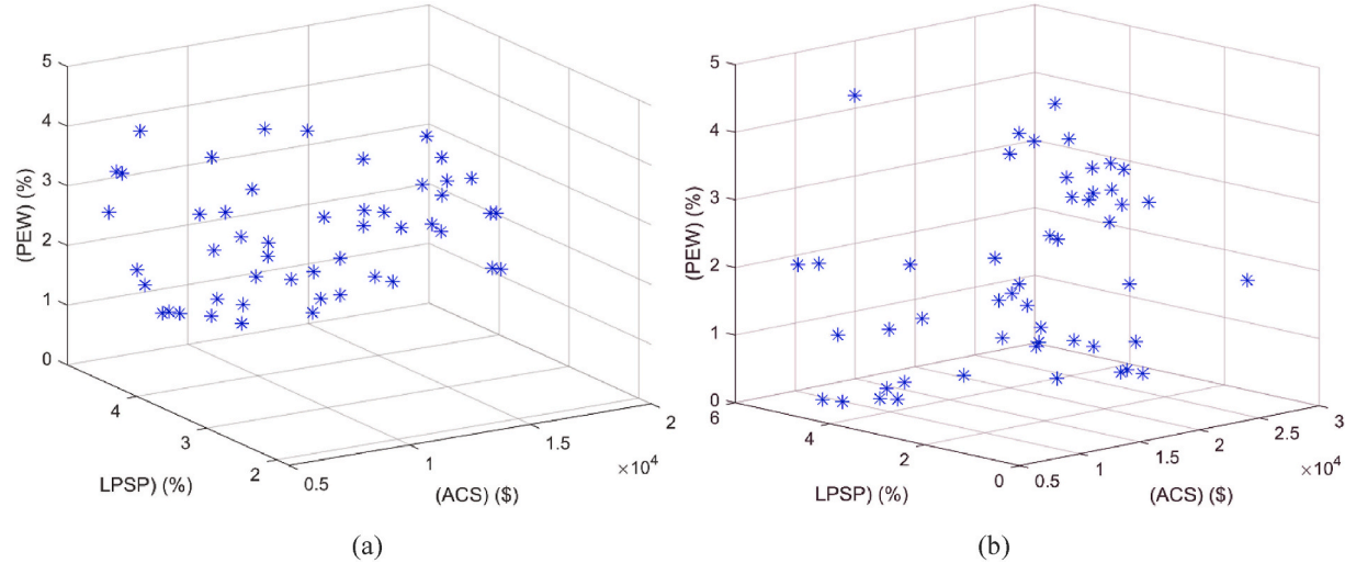
Fig. 8. The Pareto front for Kahramanmaraş (a) Scenario 1 (b) Scenario 2.
