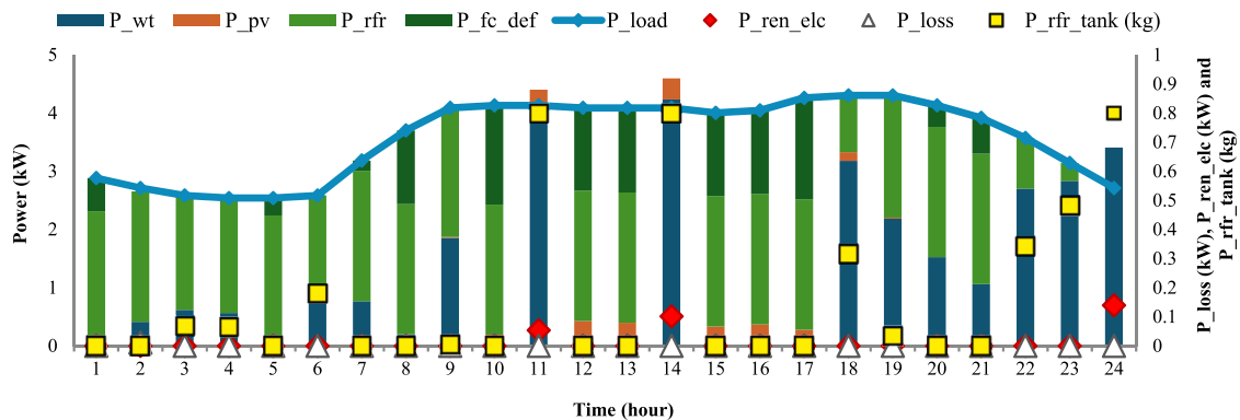
Fig. 14. Energy flow for Çeşme according to Scenario 1 of a winter day.
