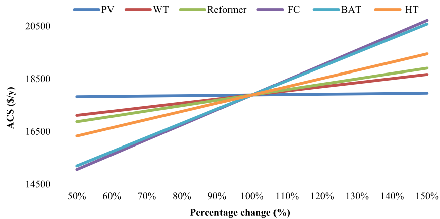
Fig. 22. Sensitivity of ACS to cost variations in PV, WT, fuel cell, battery, and HT (Scenario 2 lowest LPSP solution for Çanakkale).
