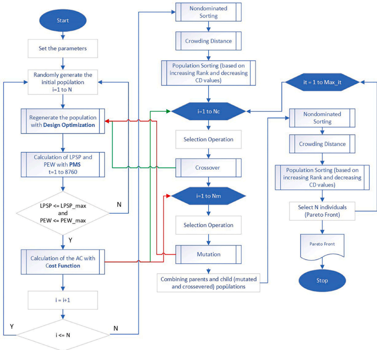
Fig. 4. Flowchart of i-NSGA-II.
