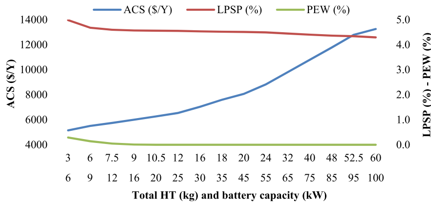
Fig. 24. The impact of increasing HT and battery capacities on ACS, LPSP, and PEW. (Scenario 2 lowest ACS solution for Çeşme).
