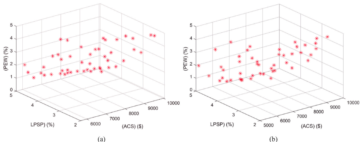
Fig. 27. The Pareto Front obtained with MOPSO for Çanakkale (a) Scenario 1 (b) Scenario 2.
