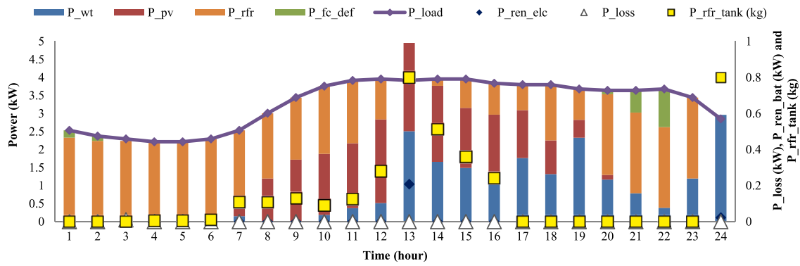
Fig. 18. Energy flow for Kahramanmaraş according to Scenario 1 of a summer day.
