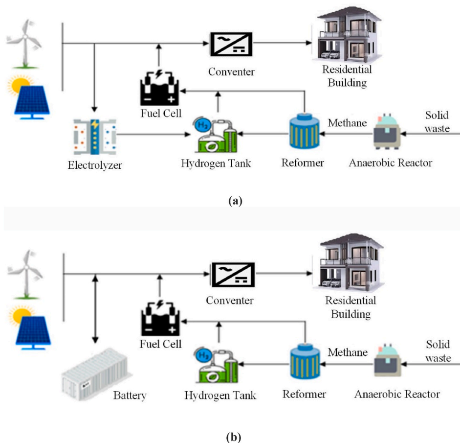
Fig. 1. Layout of the designed off-grid HRES (a) Scenario 1: HRES with hydrogen storage only (b) Scenario 2: HRES with both battery and hydrogen storage.
